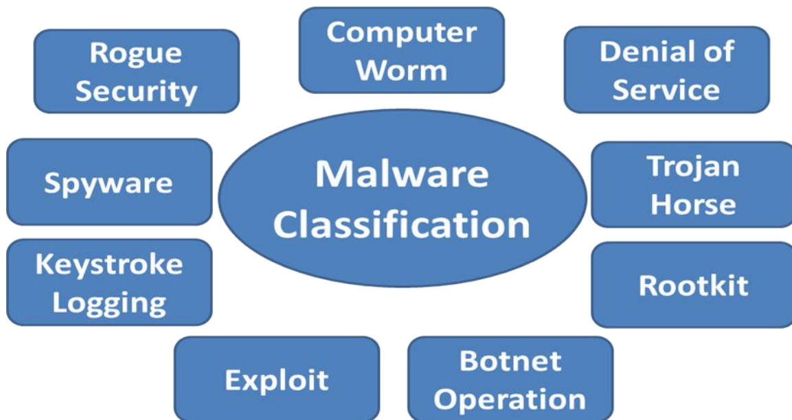
Figure 1. Malware Classification
