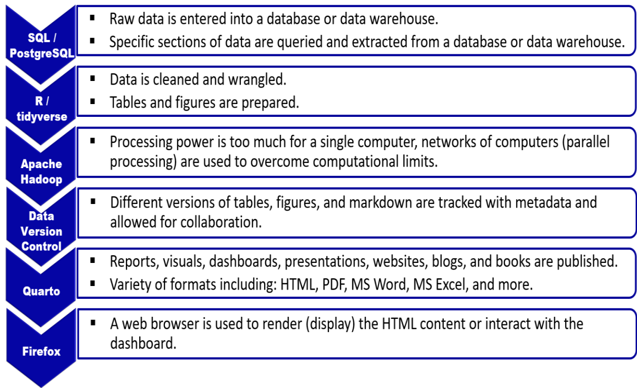
Figure 1. The OSS workflow of a data scientist.
